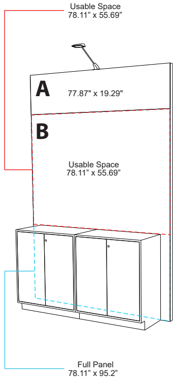
OPTION 1 No Monitor
