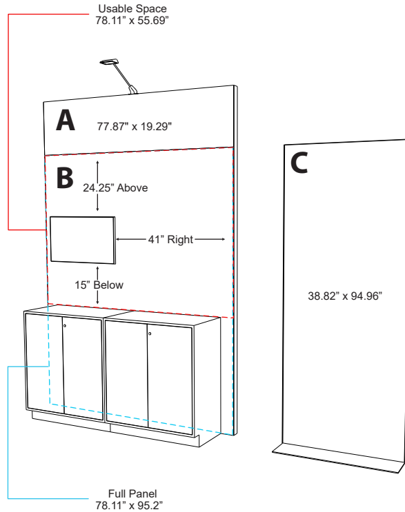
OPTION 2A / 2B Optional 32" or 40" Monitor
